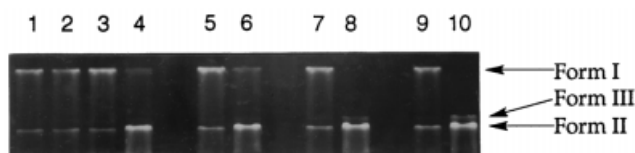
Figure 2. Comparison of \Phi\text{x} 174 cleavage efficiency between Clip-Phen, 1 , 4 , and 5 (1 \mu\text{M} ) in the presence of \text{CuCl}_2 (1 \mu\text{M} ) and MPA (5 mM); lane 1: control, no complex, no MPA; lane 2: control, no complex, with MPA; lanes 3, 5, 7, and 9: Clip-Phen, 1 , 4 , and 5 , respectively, without addition of Cu; lanes 4, 6, 8, and 10: Clip-Phen, 1 , 4 and 5 , respectively, in the presence of Cu
