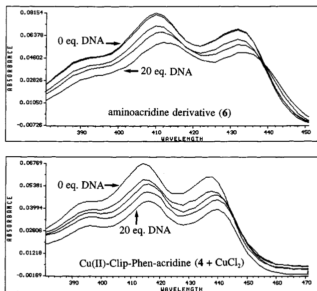
Figure 5. UV/Vis titration of 6 (top) and 4 + CuCl 2 (bottom) (all 10 \mu M) against calf-thymus DNA (0, 1, 4, 12, and 20 base-pair equivalents) in phosphate buffer (pH = 7.2) in the presence of NaCl (50 mM) and MgCl 2 (10 mM)
