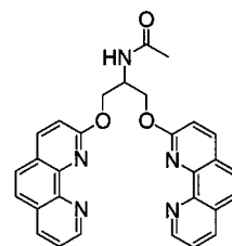
Figure 1. N -Acetyl Clip-Phen ( 1 )
