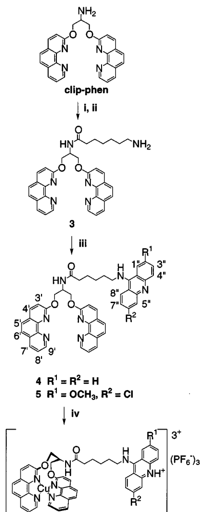
Scheme 1. Synthesis of ligands 4 and 5 , and their corresponding Cu^{II}/PF_6^- complexes; conditions: (i) 6-BOC-amino-1-hexanoic acid, EtOCOCl ; (ii) 25% CF_3COOH in CH_2Cl_2 ; (iii) appropriate 9-phenoxyacridine, CH_3CN , 10 equiv. CH_3COOH ; (iv) Cu(OAc)_2 \cdot 2 H_2O , MeOH, then NH_4PF_6 .
