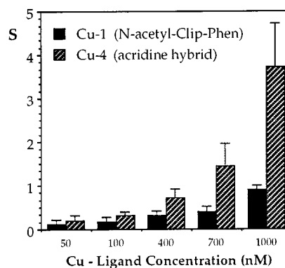
Figure 3. Concentration dependence of \Phi\text{x} 174 cleavage efficiency for 1 (solid) and 4 (hatched) in the presence of equimolar \text{CuCl}_2
