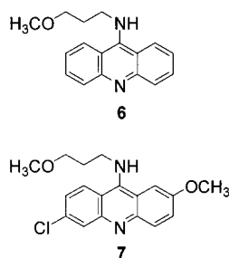
Figure 4. Alkylaminoacridine derivatives 6 and 7
